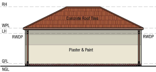
SIDE ELEVATION
