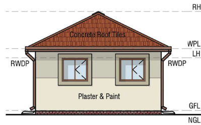
BACK ELEVATION
